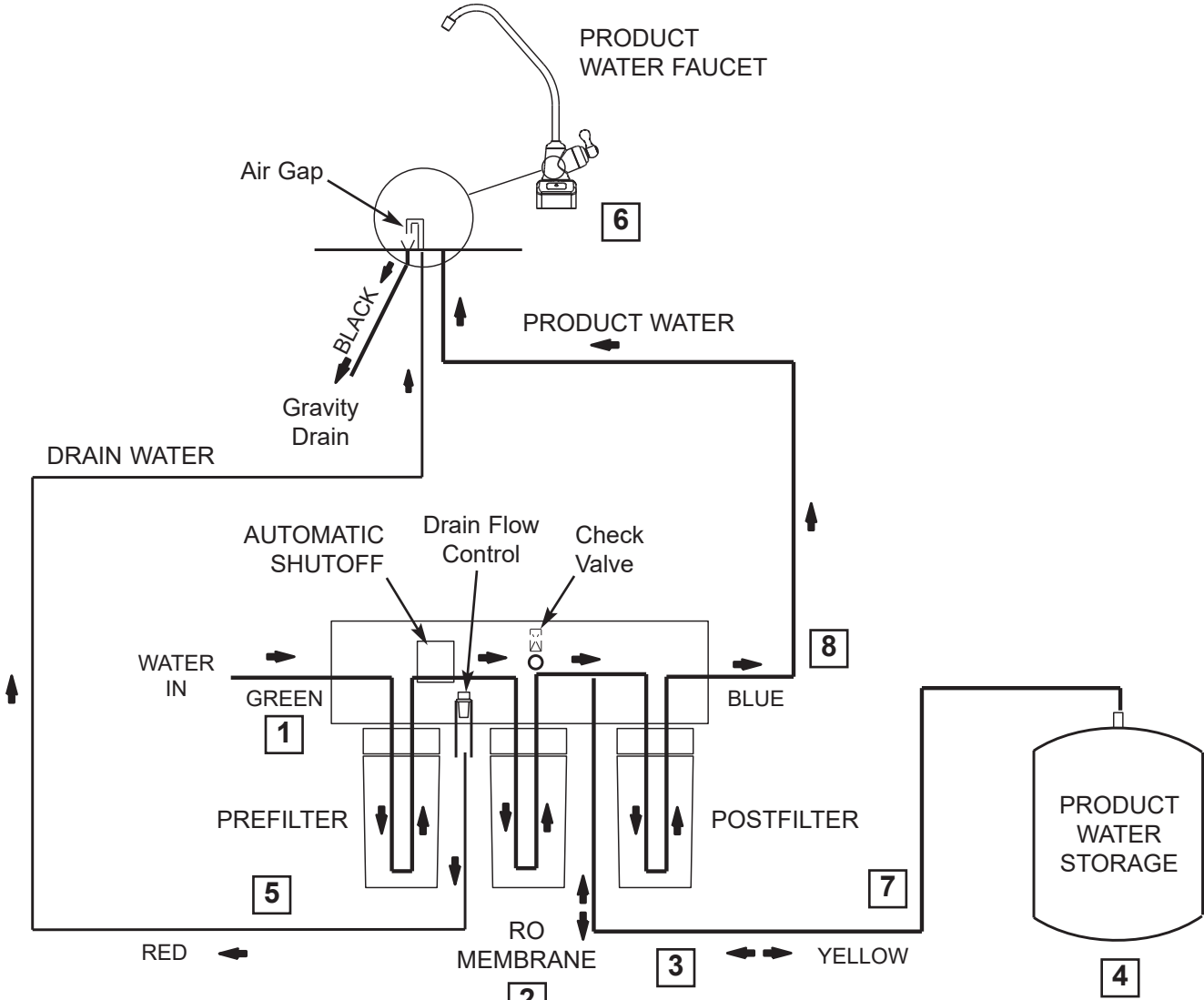
Reverse Osmosis Water Flow Schematic
